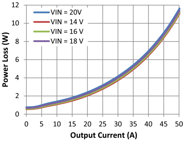
Figure 6. Power Loss vs. Input Voltage
