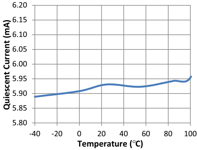
Figure 16. Quiescent Current vs. Temperature
