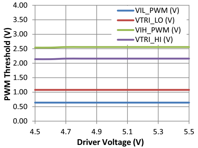
Figure 13. PWM Threshold vs. Driver Voltage
