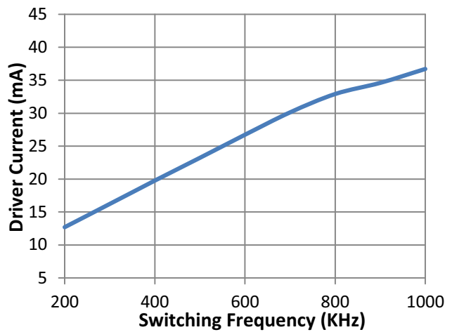
Figure 9. Driver Supply Current vs. Switching Frequency
