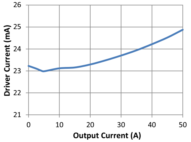
Figure 11. Driver Current vs. Output Current
