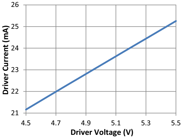
Figure 10. Driver Current vs. Driver Voltage
