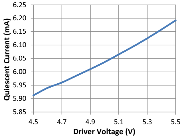
Figure 15. Quiescent Current vs. Driver Voltage
