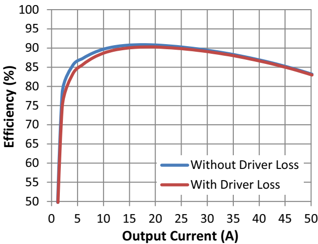
Figure 8. Efficiency vs. Output Load
