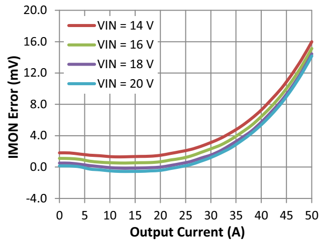
Figure 21. I_{MON} Accuracy vs. Input Voltage
