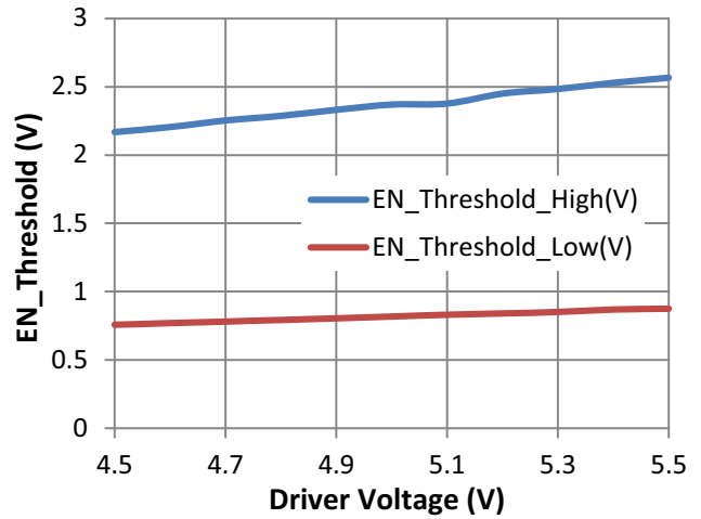
Figure 17. EN Threshold vs. Driver Voltage
