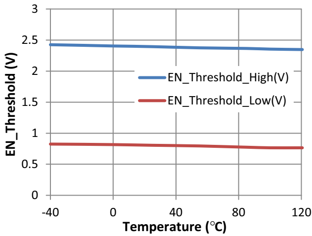
Figure 18. EN Threshold vs. Temperature
