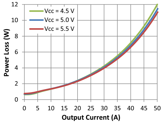
Figure 7. Power Loss vs. Driver Voltage
