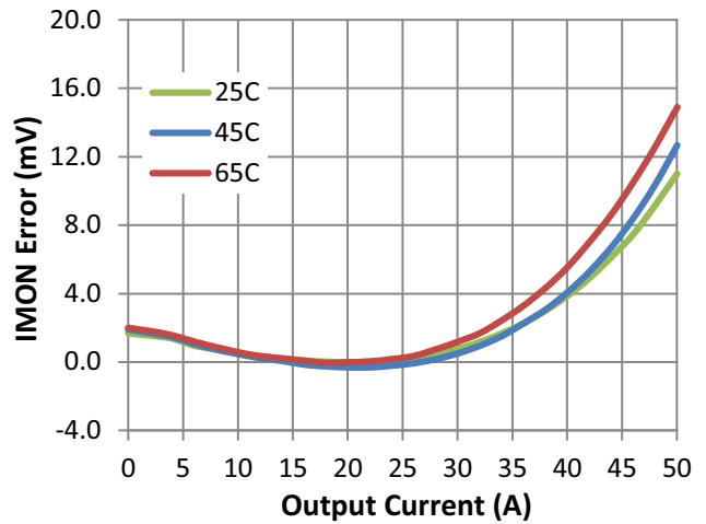
Figure 19. I_{MON} Accuracy vs. Temperature
