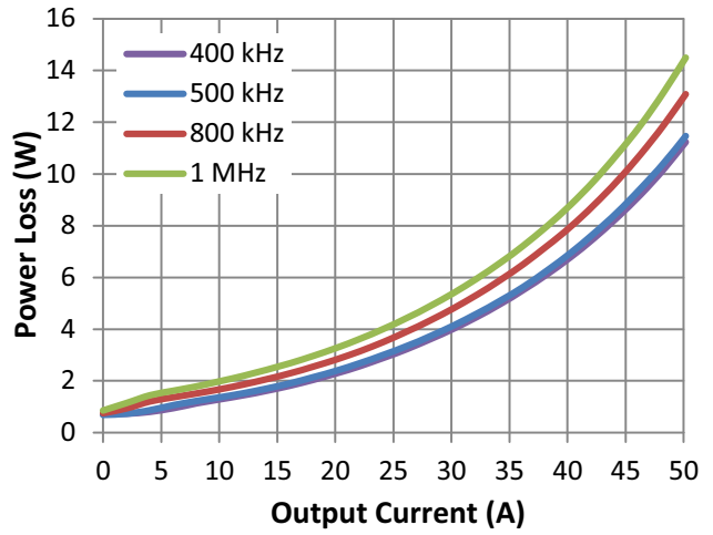
Figure 5. Power Loss vs. Switching Frequency
