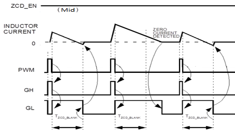
Figure 25. Timing Diagram – 3-state PWM Controller, No ZCD (b)
