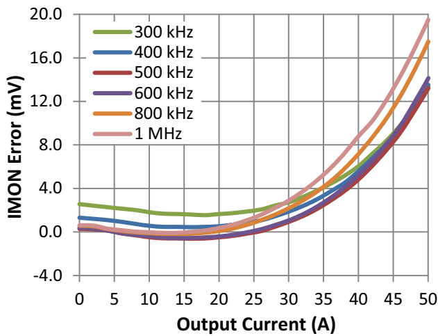
Figure 20. I_{MON} Accuracy vs. Switching Frequency
