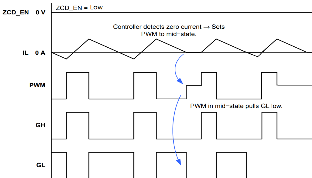
Figure 26. Timing Diagram – 3-state PWM Controller, with ZCD
