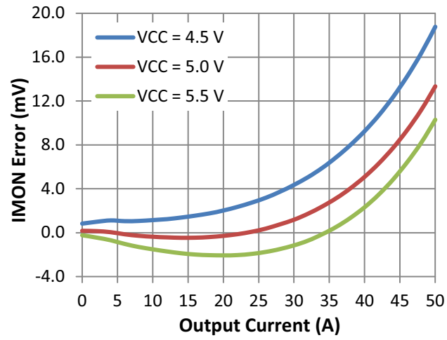
Figure 22. I_{MON} Accuracy vs. Driver Voltage
