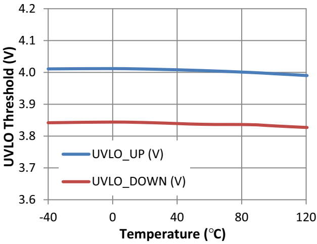
Figure 12. UVLO Threshold vs. Temperature
