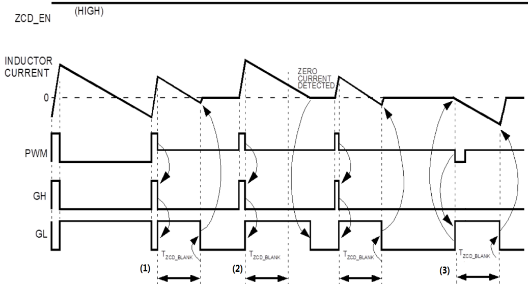
Figure 24. Timing Diagram – 3-state PWM Controller, No ZCD (a)
