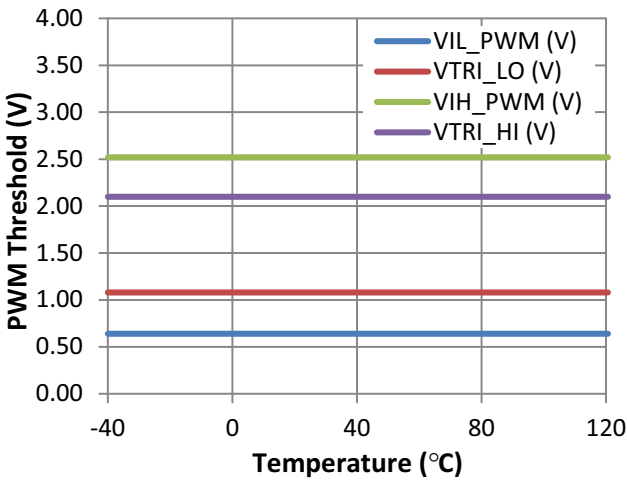
Figure 14. PWM Threshold vs. Temperature
