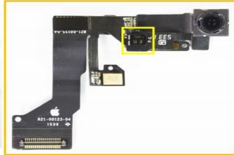
proximity sensor (mnf. unknown) 2.78 mm x 2.38 mm x 1.28 mm
